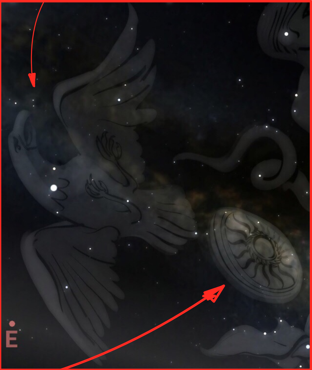
Eagle & Shield Constellations
